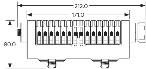
Fixed Housing
