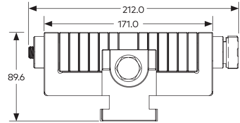
Free Housing
